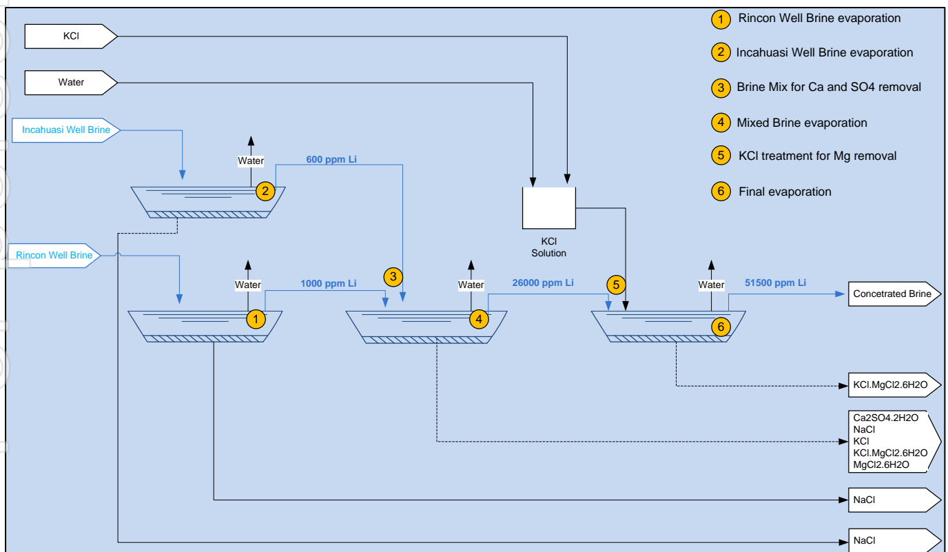
Figure 1: Brine-Blending Evaporation Process Flowsheet
